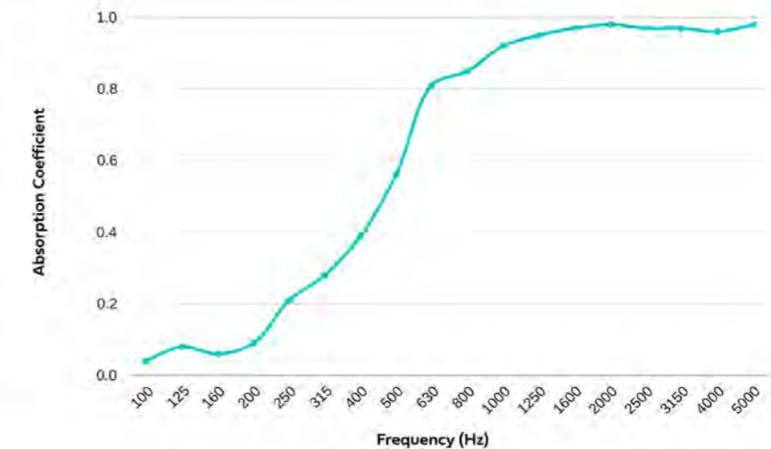
24mm Sound Absorption Coefficient
